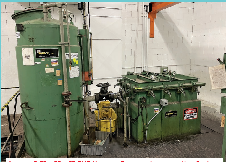
Imprex S-39 x 53 x 62 OHO Vacuum Pressure Impregnation System
